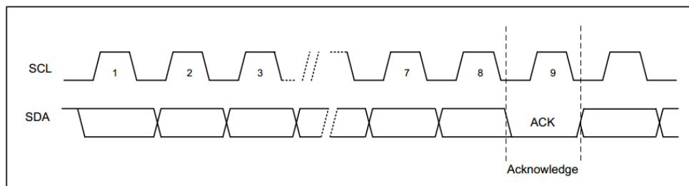
Figure 3 Output Acknowledge
